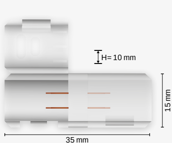
2490036 Conector Conector | Connector
